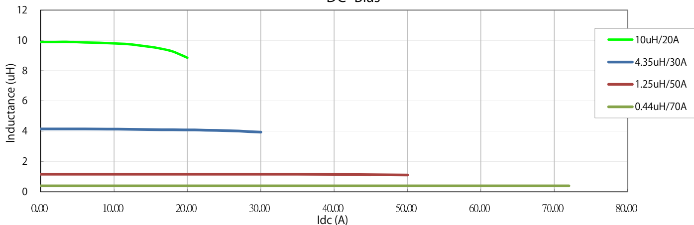
DC Bias
